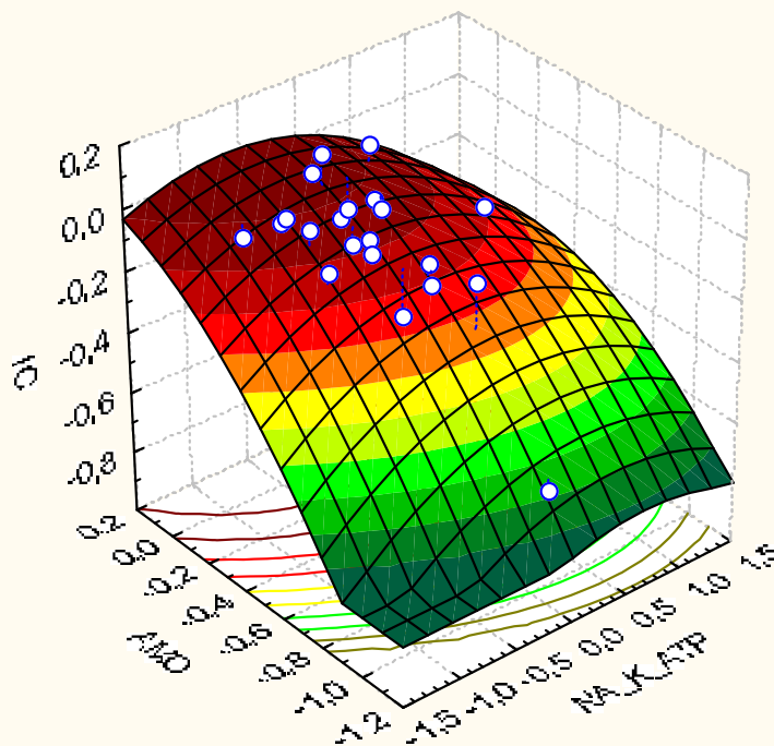
Quadratic Surface NA_K_ATP vs. AMO vs. IC (Casewise deletion of missing data)
