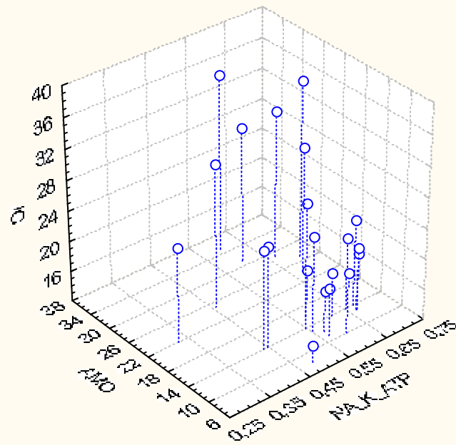
3D Scatterplot NA_K_ATP vs. AMO vs. IC (Casewise deletion of missing data)
