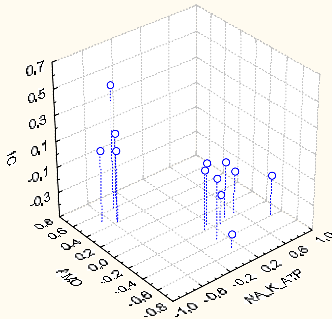
3D Scatterplot NA_K_ATP vs. AMO vs. IC (Casewise deletion of missing data)
