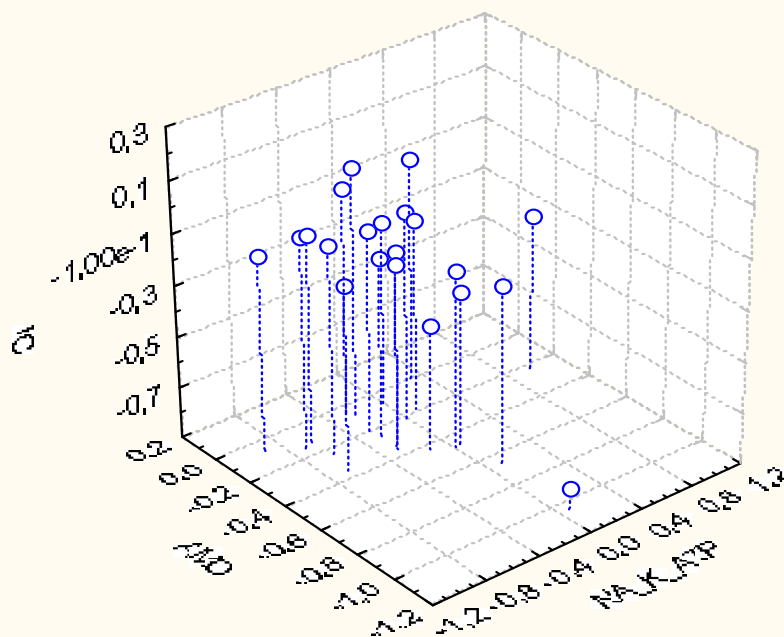
NA_K_ATP vs. AMO vs. IC (Casewise deletion of missing data)
