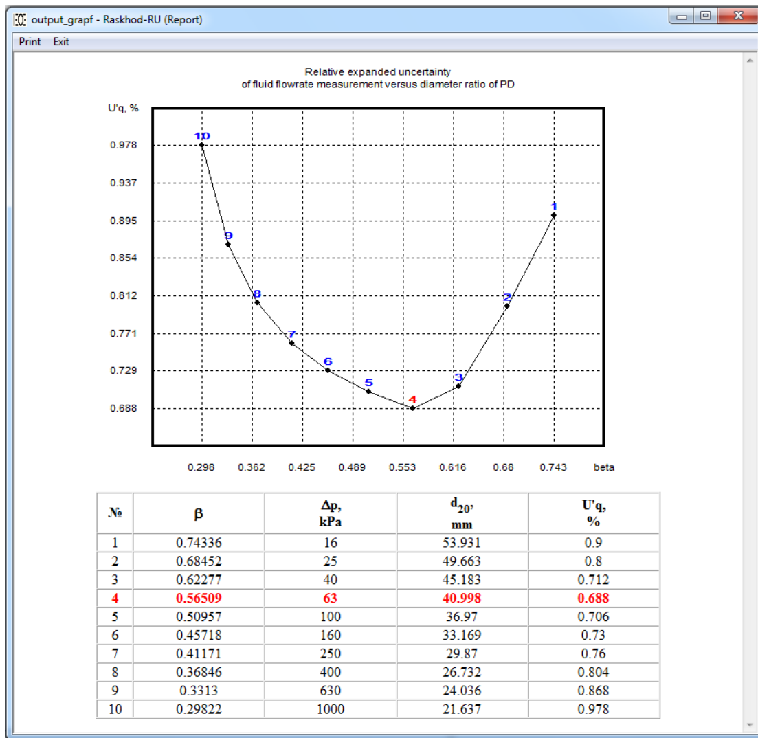
Fig. 5. The curve of relative expanded uncertainty of fluid flowrate measurement versus diameter ratio of the primary device together with the table of the corresponding values.
