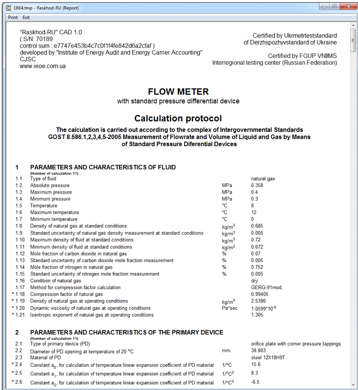
Fig. 4. Flowmeter calculation protocol (a part of the protocol).
