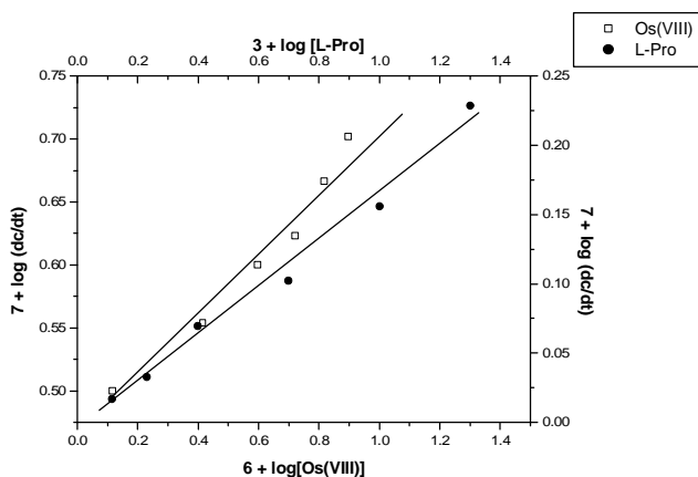
Fig. 4. Plot between rate \log[Os(VIII)] vs. \log(dc/dt) and \log[L\text{-Pro}] vs. \log(dc/dt) for oxidation of L-Pro at 308 K
