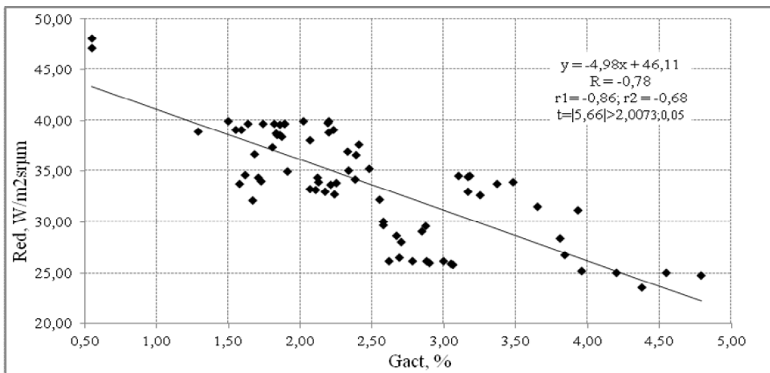
Fig. 2. Linear statistical dependence of G_{act} and the spectral brightness in the Red channel (08.03.2013) Landsat 8 OLI
