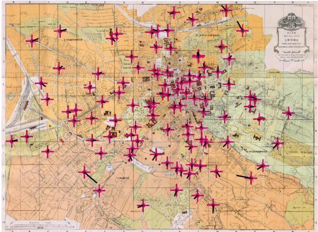
Fig. 5. Vectors of displacements on the plan of Lviv in 1894
