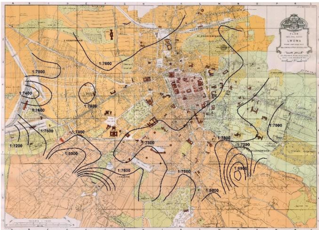
Fig. 7. Isolines of scale variations with an impact radius of 800 m, built with a step of 200 m
