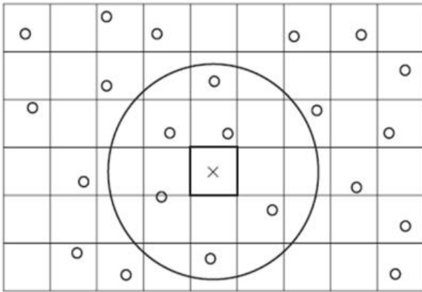
Fig. 6. Six points inside a circle, calculating the scale or rotation angle of the cell in the center
