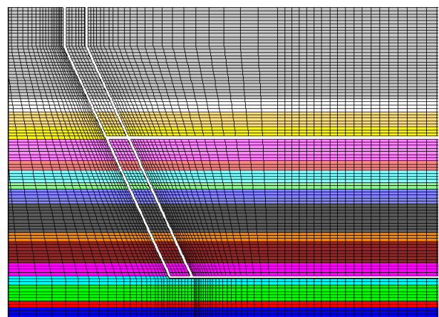
Fig. 2. Simulation model of the process of digging the tunnels in the II section of Seam 14 of the Ha Lam Coal Mine
