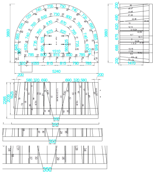
Fig. 3. Passport of drilling and blasting operations in rocks enclosing a pair of inclined shafts and crosscuts [22]
