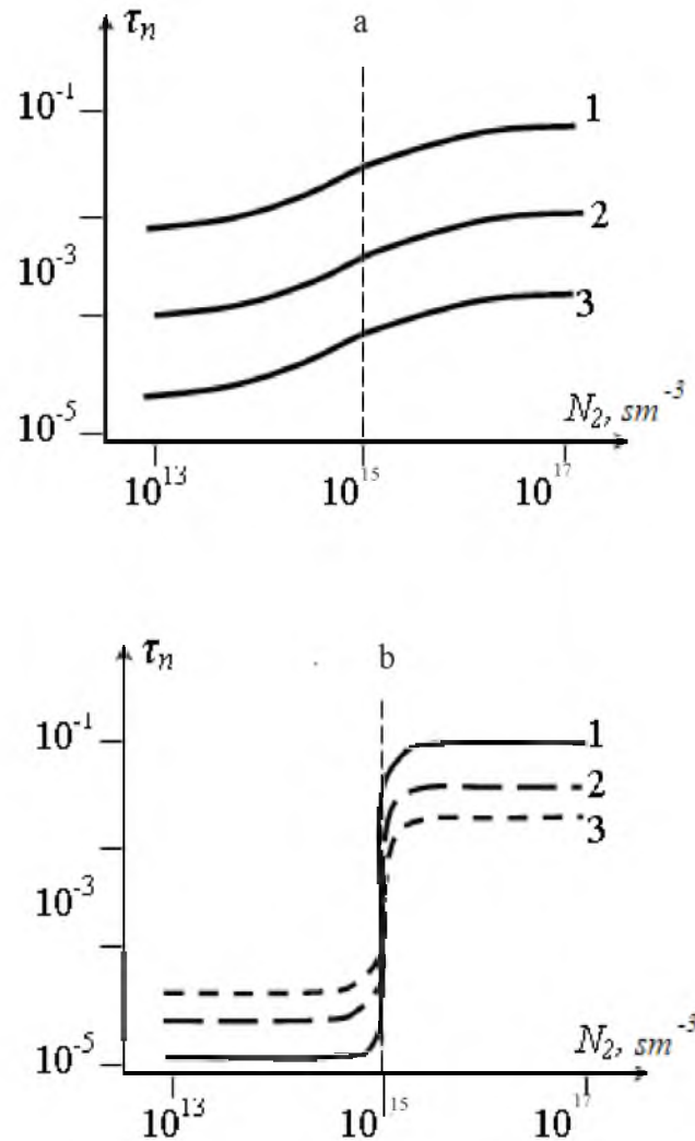
Fig. 2.1. The change of the lifetime of electrons when the concentration of R-centers for levels of photoexcitation: 1 – 10^{14} , 2 – 10^{15} and 3– 10^{17} \text{ sm}^{-3}\text{s}^{-1} . A – the calculation was performed for positive, B - for negatively charged centers of first grade.
