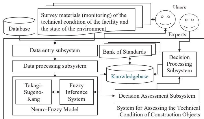
Fig. 3. The scheme of integration of the artificial neural network Takagi-Sugeno-Kang in the system for assessing the technical condition of construction objects
