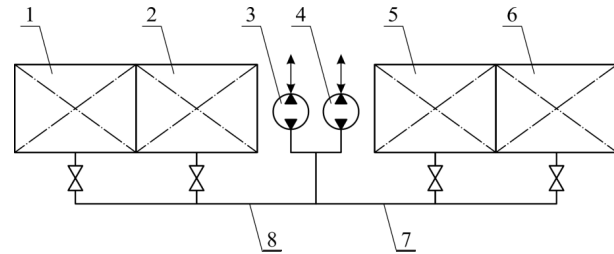
Fig. 1. Schematic diagram of the arrangement of cargo tanks of a PSV class vessel intended for transportation of drilling slurry (fragment): 1, 2, 5, 6 – cargo tanks; 3, 4 – cargo pumps; 7, 8 – lines for receiving/pumping out drilling slurry
