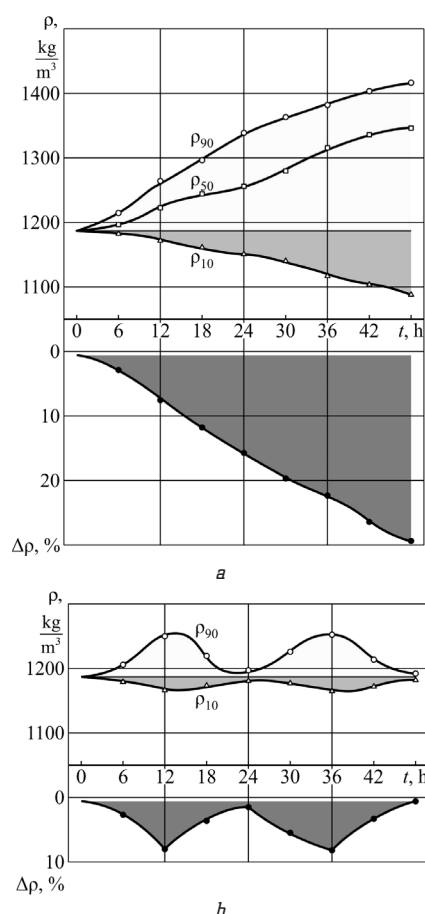
Fig. 3. Change in density, \rho , and sedimentation stability, \Delta\rho , of the drilling slurry depending on time: a – transportation without upgrading the system design; b – transportation with additional X-shaped circulation
