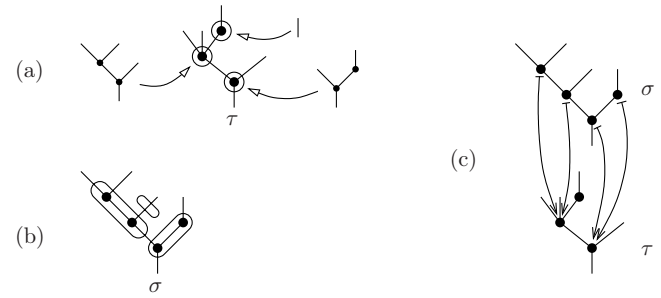
Fig. 4. Three pictures of a map in \mathbf{Tree}_4
