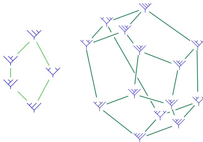
Fig. 2. Tamari order on T_3 and T_4
