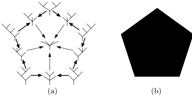
Fig. 7. (a) The category of 4-leafed stable trees, and (b) its classifying space
