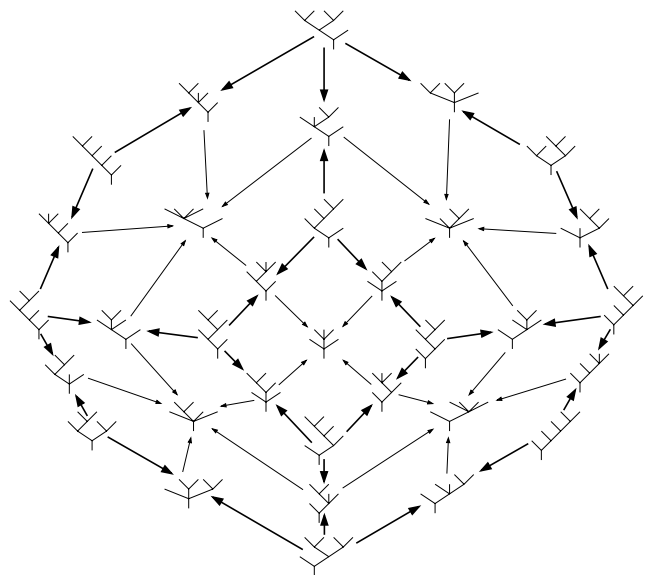
Fig. 8. About half of the category of 5-leafed stable trees
