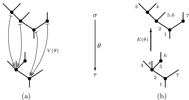
Fig. 10. Effect of a certain map of 4-leafed trees on (a) vertices and (b) edges
