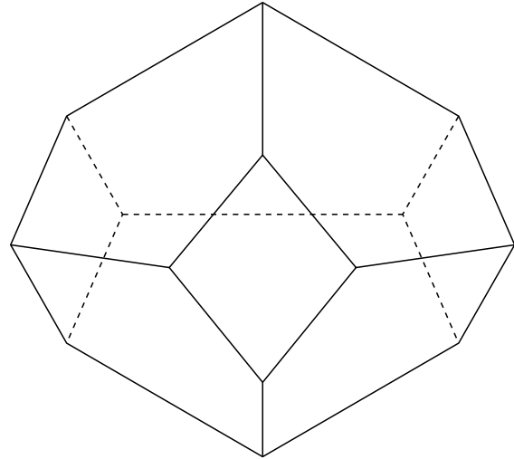
Fig. 9. Classifying space of the whole category of 5-leafed stable trees
