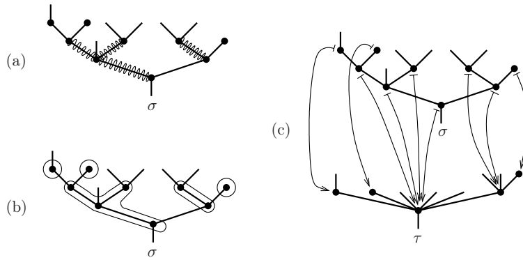
Fig. 5. Three pictures of an epic in \mathbf{Tree}_6
