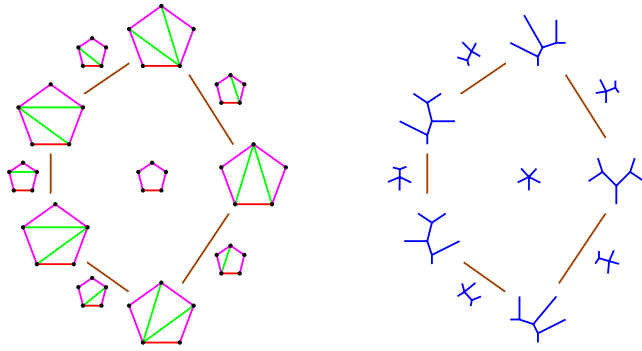
Fig. 3. Two views of the associahedron \mathcal{A}_3
