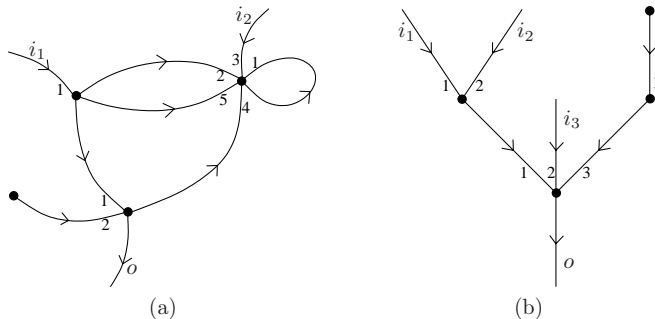
Fig. 1. (a) Input-output graph with 4 vertices and 2 input edges i_1, i_2 , (b) combinatorial tree with 4 vertices and 3 input edges i_1, i_2, i_3 . In both, the numbers indicate the order on the edges arriving at each vertex
