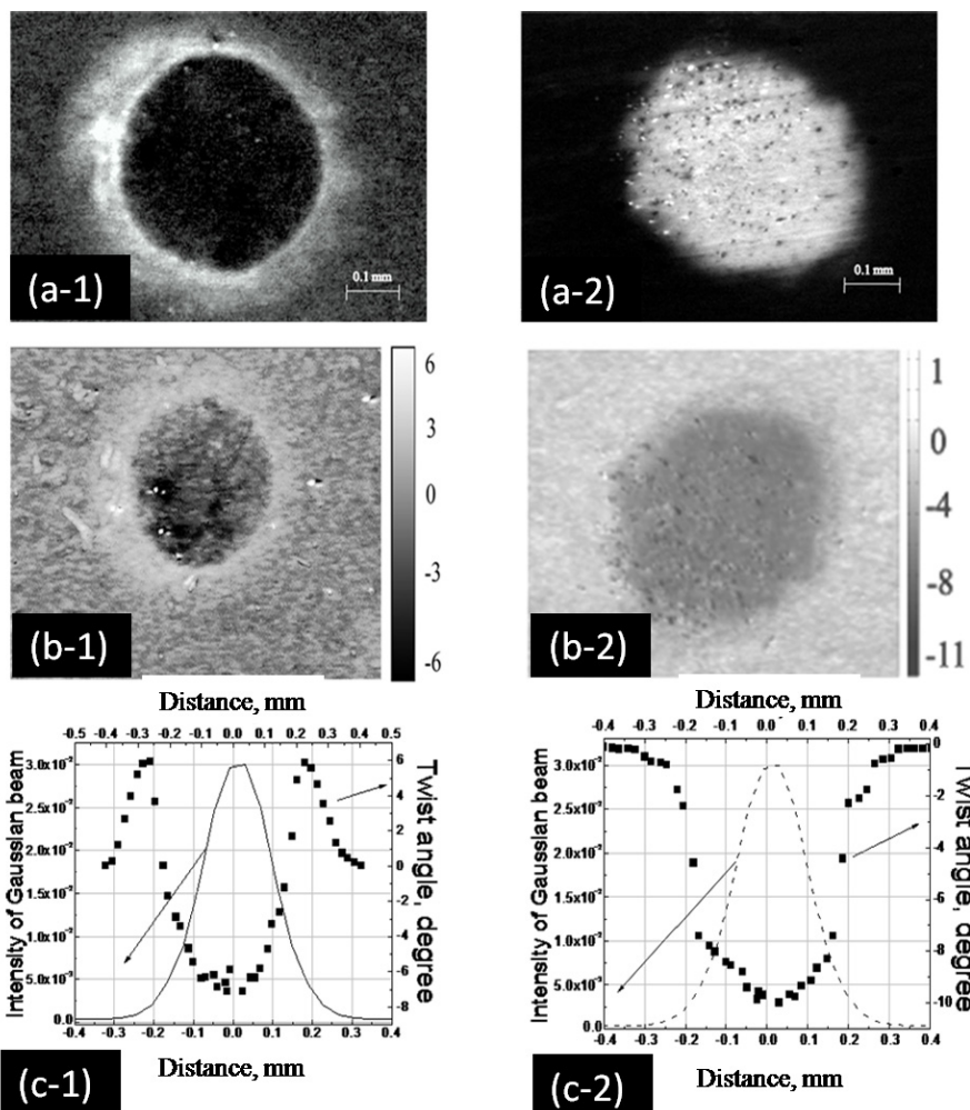
Fig. 1. a) Images of twist structures in the crossed polarizers. \tau_{exp} = 30 min (a-1) LC 5CB, (a-2) LC E7. b) spatial distributions \psi(x, y) in the cells with LC 5CB (b-1) and LC E7 (b-2). c) The cross section of the spatial distribution of \psi(x, y) . The profiles of the exciting polarization beam with the Gaussian intensity distributions. (c-1) LC 5CB, (c-2) LC E7
