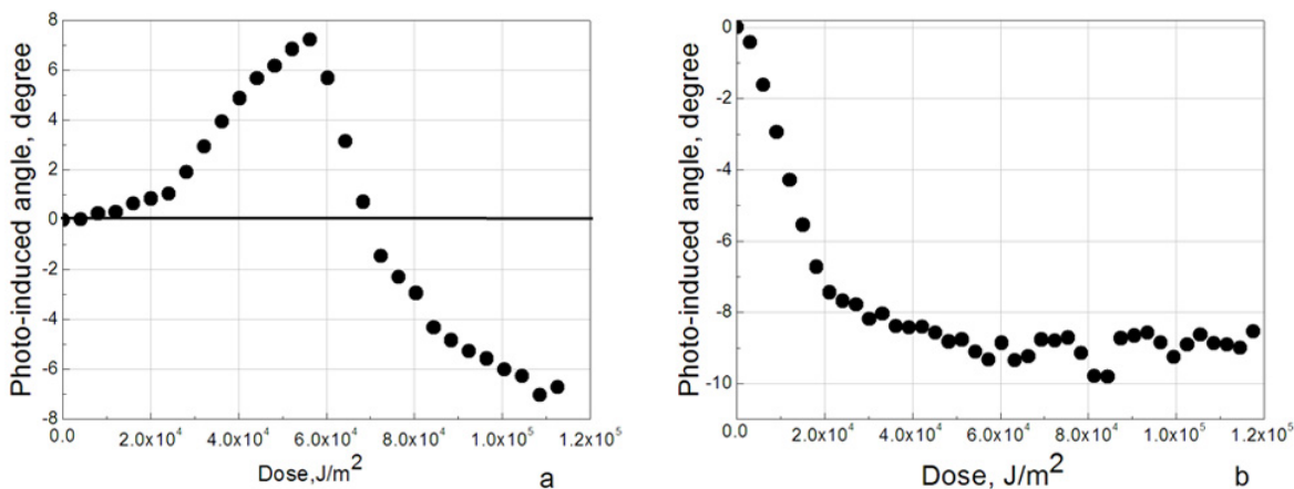
Fig. 2. Dependence of the photoinduced reorientation of the directors of LCs 5CB (a) and LCs E7 (b) on the irradiation on chalcogenide glass As_{20}Se_{80}
