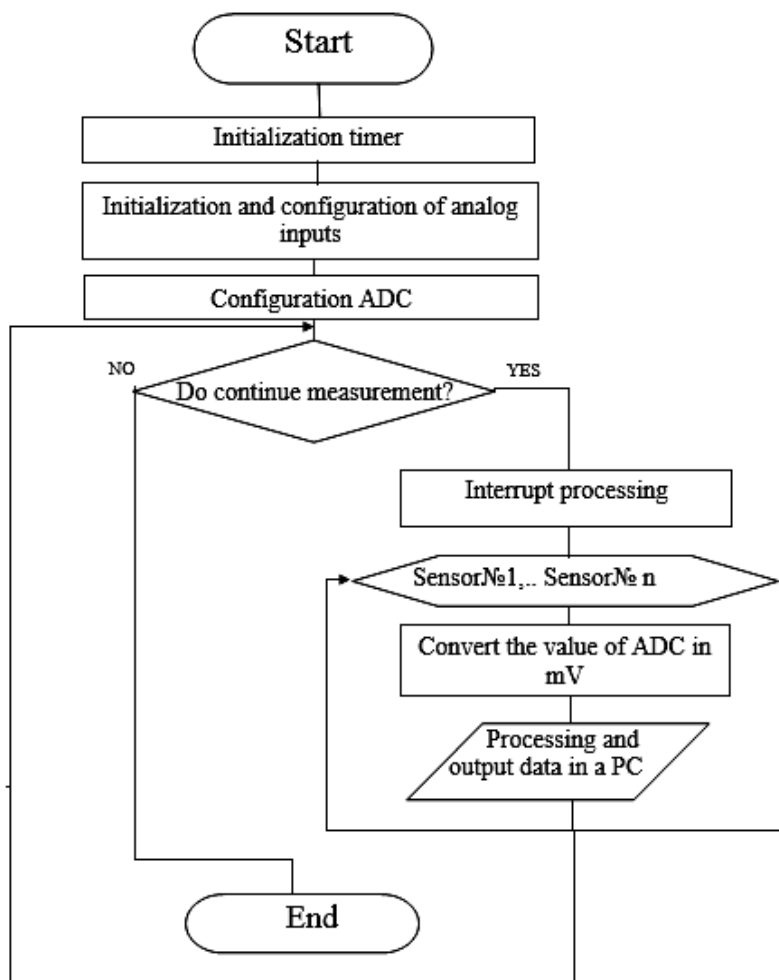
Fig. 3 Block diagram of the algorithm of the GA
