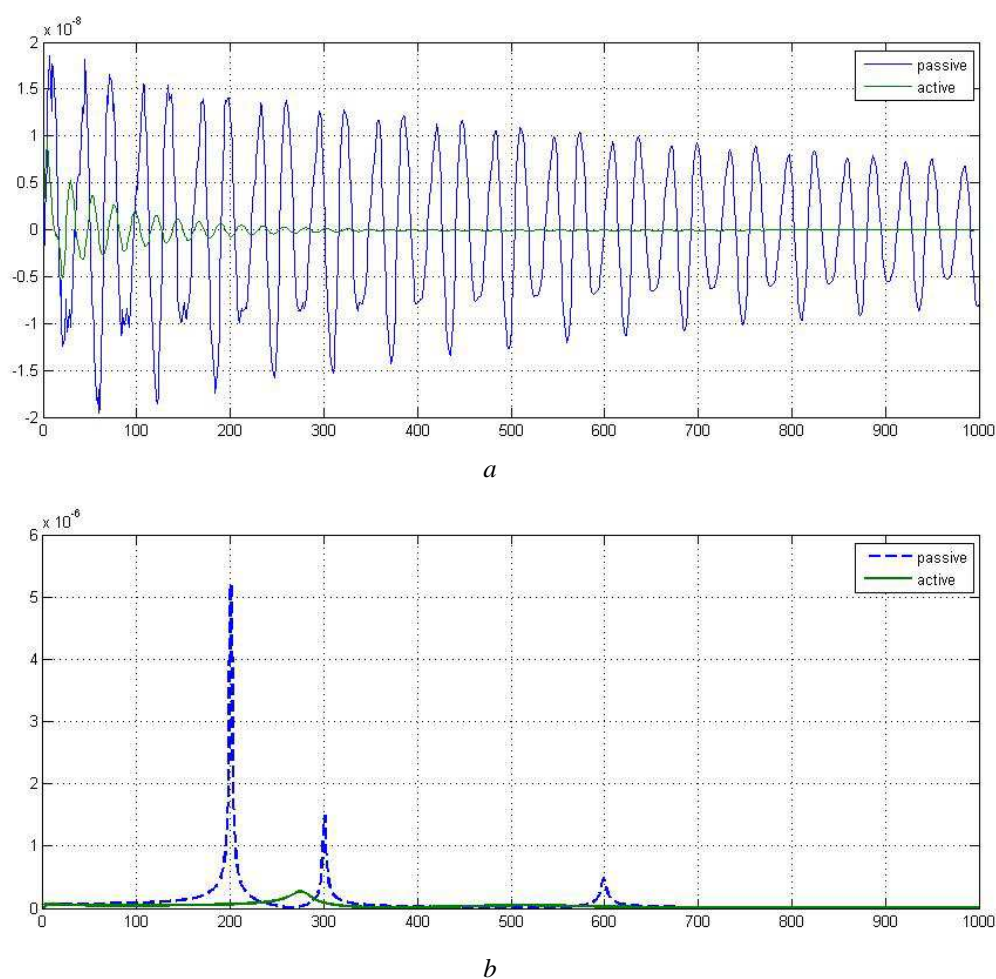
Fig. 3. Reaction of the beam to a shock load (a) and frequency response (b) for an optimal value of the amplification coefficient G_{opt} = 10^{-4}
