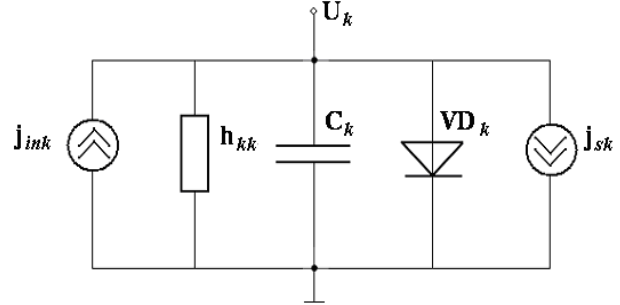
Fig. 1. The universal environment of the equivalent scheme of the aggregated model
