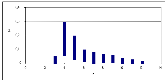
Fig. 4. (r / d_0) values where H_0: d = d_0 cannot be rejected in model: (1 - 2\cos w_r L + L^2)^d x_t = u_t ; u_t is AR(1) u_t
