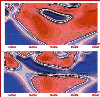
Geophysics
