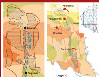
Geoecology
