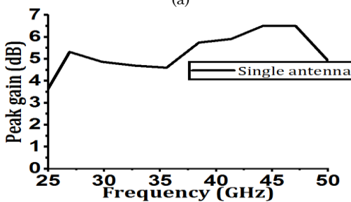
Fig. 4 – Proposed single element antenna (a) S_{11} (b) gain
