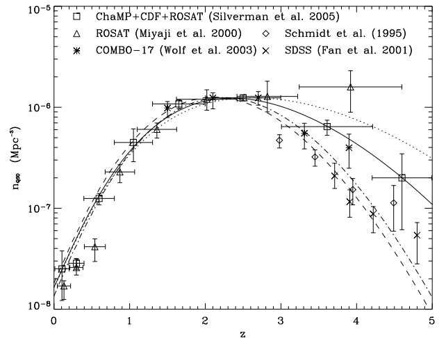
Fig. 1. The dependence of QSOs co-moving number density on redshift: theoretical curves versus observational data. Solid line shows the best fitting model with M = 8 \cdot 10^{11} h^{-1} M_\odot and e_m = 0.38 . Dashed and dash-dotted lines present the models with the same protogalactic clouds masses M = 4 \cdot 10^{12} h^{-1} M_\odot , but different ellipticities, e_m = 0.2 and e_m = 0.17 , respectively. Dotted line shows the co-moving space number density of QSOs for the model with M = 3 \cdot 10^{11} h^{-1} M_\odot and e_m = 0.5 .
