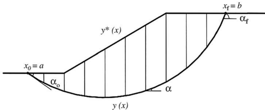
Fig. 1. Collapse mechanism in the limit equilibrium approach
