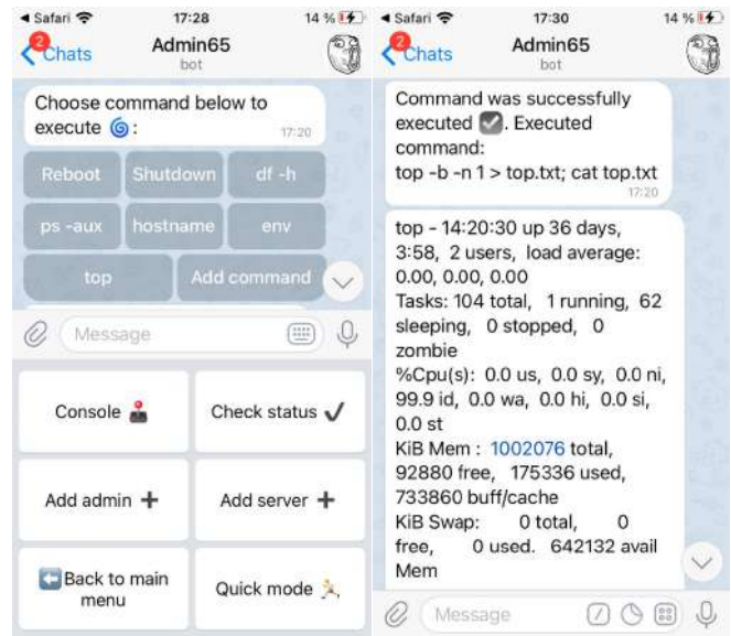
Fig. 6. Quick mode commands and user's account menu
