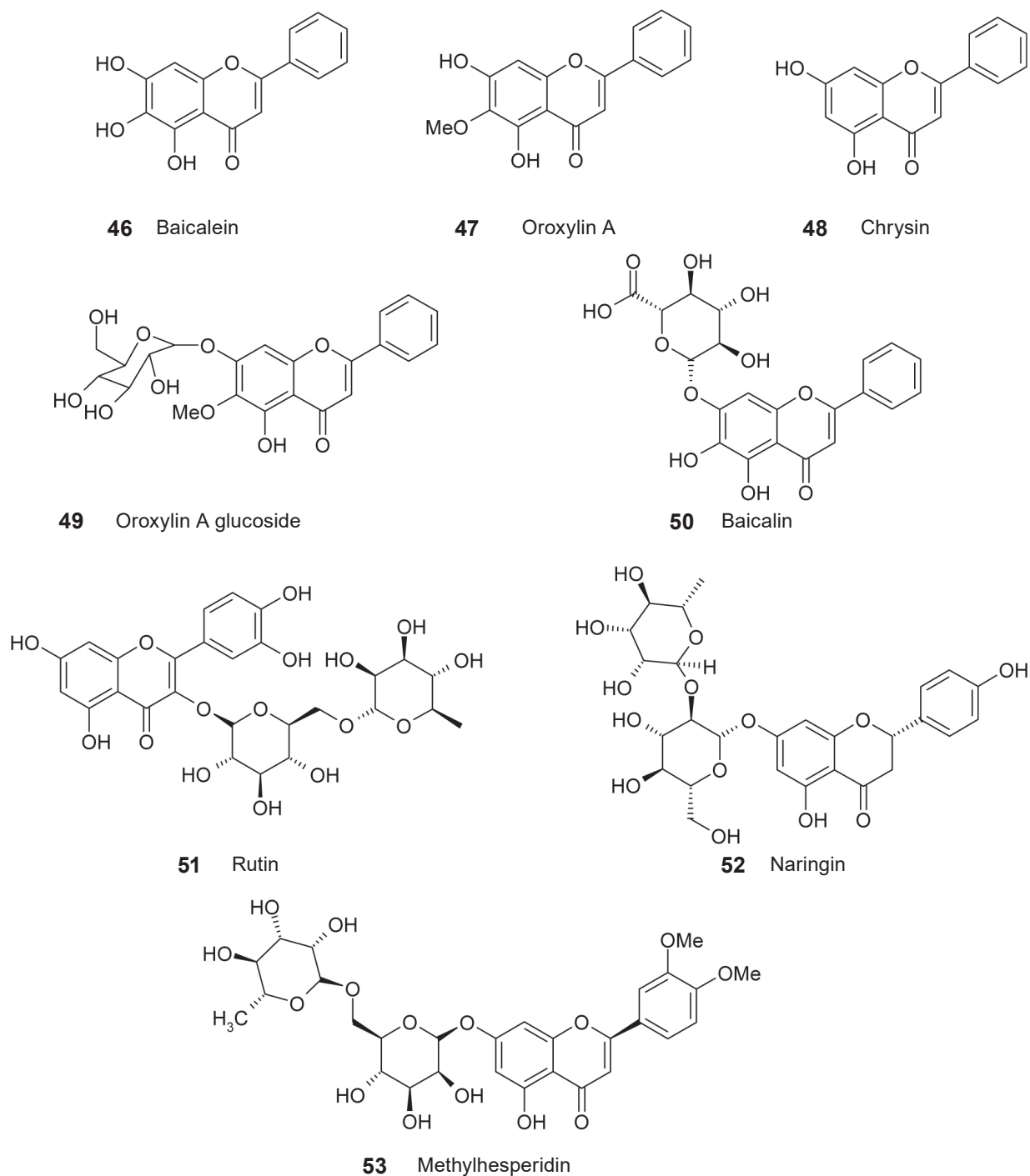
Fig. 7. Flavonoids, which block the furin and other PCs activities
