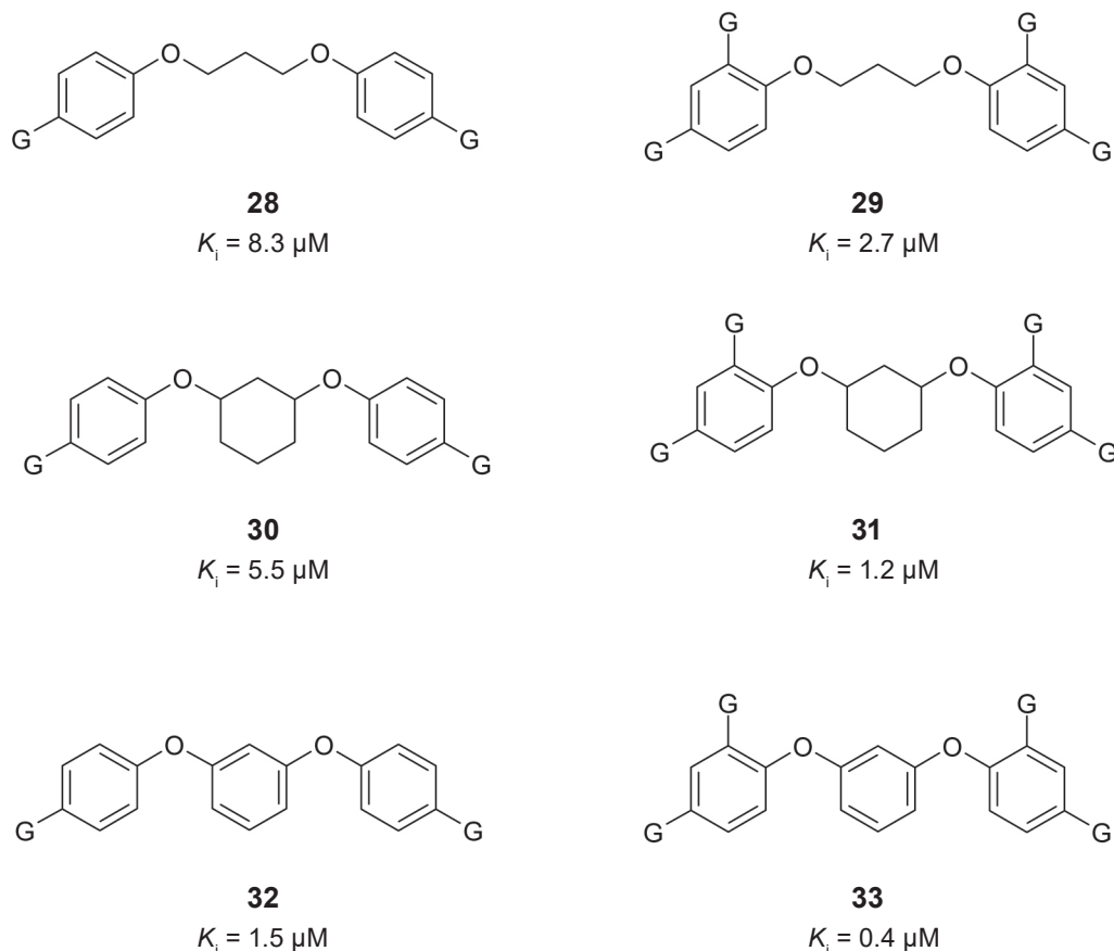
Fig. 3. Structure and activity of bis-guanidinophenyl esters ( G - guanidine group) [40]
