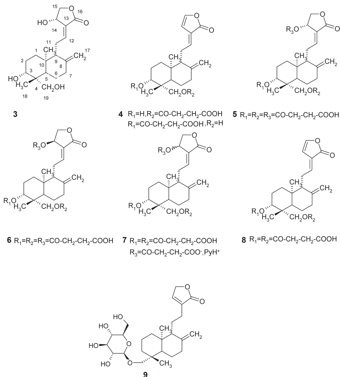
Fig. 2. Chemical structures of non-peptide andrographolide-based furin inhibitors: 3 – andrographolide; 4 – 14-dehydroandrographolide succinic acid monoester (DASM); 5 – succinic ester of andrographolide-1 (SEA-1); 6 – SEA-2; 7 – SEA-4; 8 – SEA-5; 9 – neoandrographolide [37]
