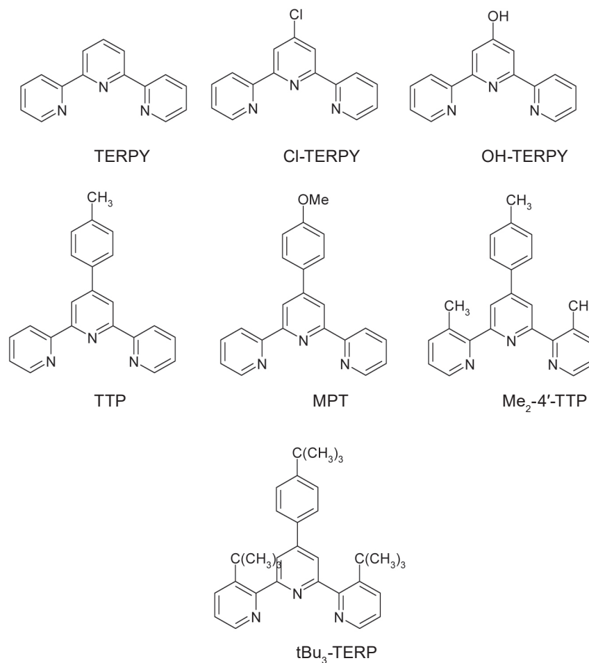
Fig. 5. Structures of terpyridine derivatives, which inhibit furin activity [42]
