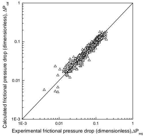
Fig. 5. Correlation plot of frictional pressure drop
