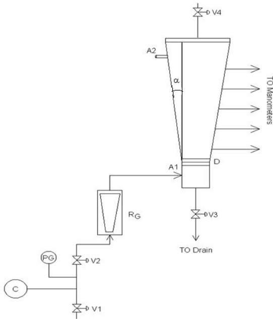
Fig. 1. Schematic diagram of experimental setup [2]:
