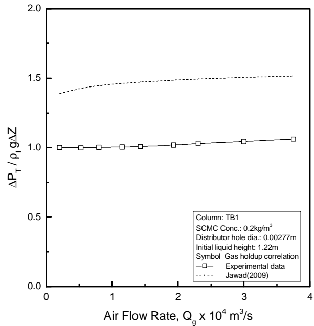
Fig. 4. Comparison of frictional pressure drop data with Jawad [22] correlation
