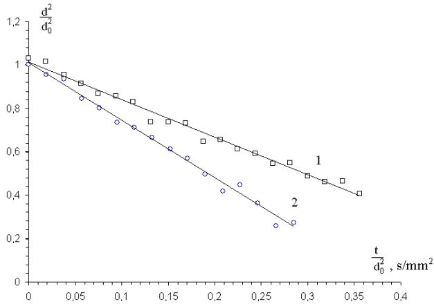
Fig.3. Squared diameters of burning droplets ( d_0 = 1.87 \text{ mm} ): ○ – Docosane; ■ – Octadecane.
