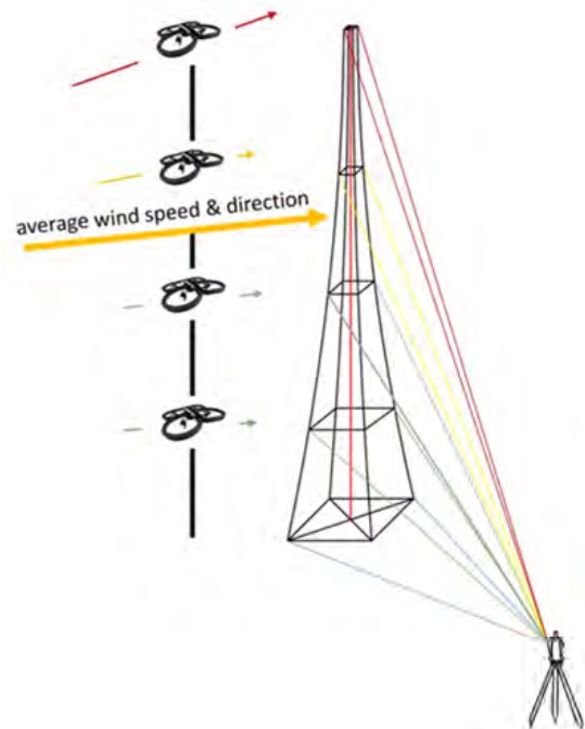
Fig. 2. The concept of angles measurements including measurement of the wind (speed and direction) by UAV
