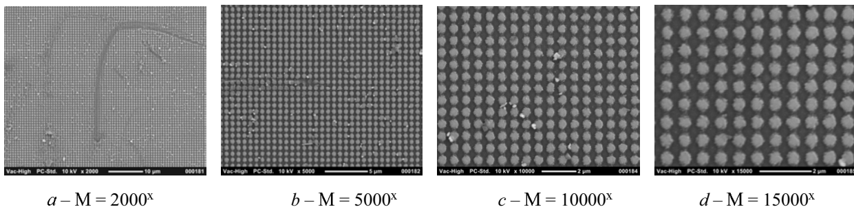
Fig. 1. Digital SEM images of the test object with a resolution r = 1425 \text{ lin/mm} at different M^x
