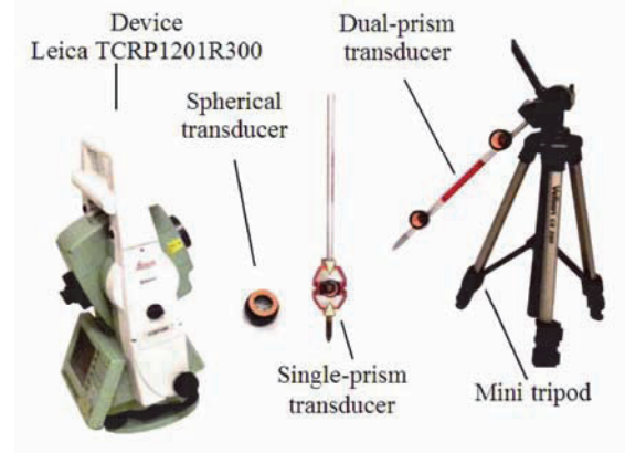
Fig. 2. Measurement system for determining the geometric parameters of building construction
