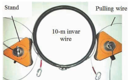
Fig. 8. Set of installation for measurement of ten-meter segments
