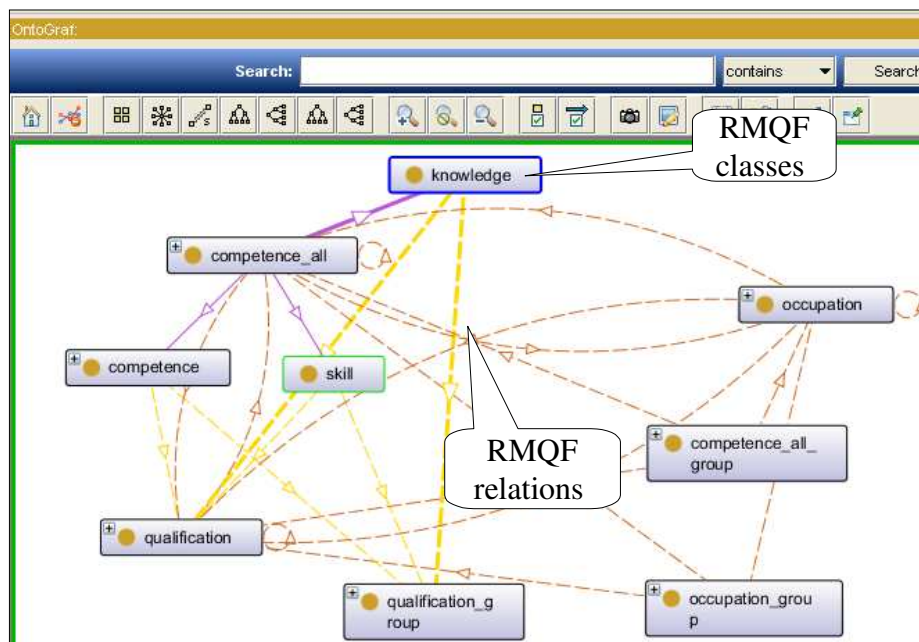
Pic. 1. RMQF main classes and relations visualized by Protégé plugin Ontograf
