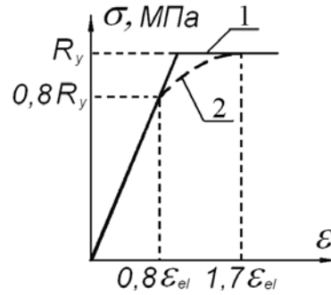
Figure 2. Diagrams « \delta - \epsilon » of steel [6]: 1 – idealized; 2 – unified.
