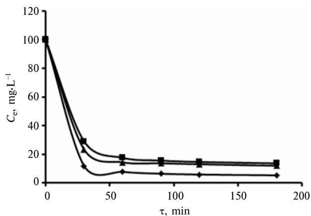
Fig. 4. The residual dyes concentration depending on the sorption time on MCS 3: ◆ – Malachite green; ■ – Congo red; ▲ – Indigo carmine
