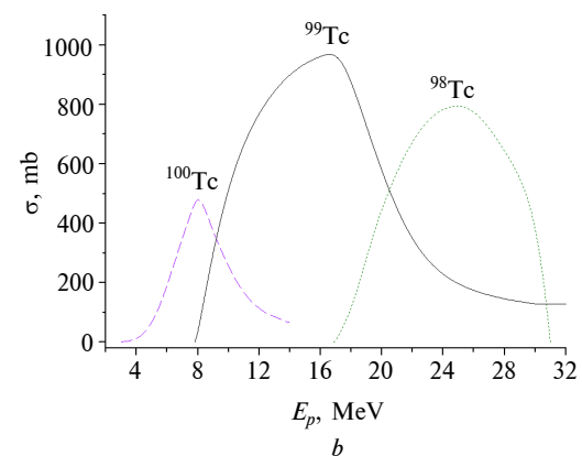
Fig. 2. The cross sections of ^{99g}\text{Tc} , ^{99m}\text{Tc} and ^{100}\text{Tc} , ^{99}\text{Tc} , ^{98}\text{Tc} ( b ) production depending on an energy of protons E_p calculated using Empire 3.2 code: ----- — ^{100}\text{Mo}(p,2n)^{99g}\text{Tc} ; — — ^{100}\text{Mo}(p,2n)^{99m}\text{Tc} ; ..... — ^{100}\text{Mo}(p,3n)^{98}\text{Tc} ; — — — — ^{100}\text{Mo}(p,2n)^{99}\text{Tc} ; - - - - - — ^{100}\text{Mo}(p,n)^{100}\text{Tc}
