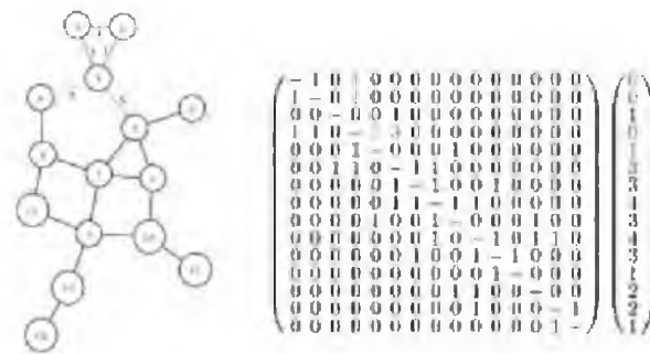
Fig. 4. SBCA algorithm after first iteration
