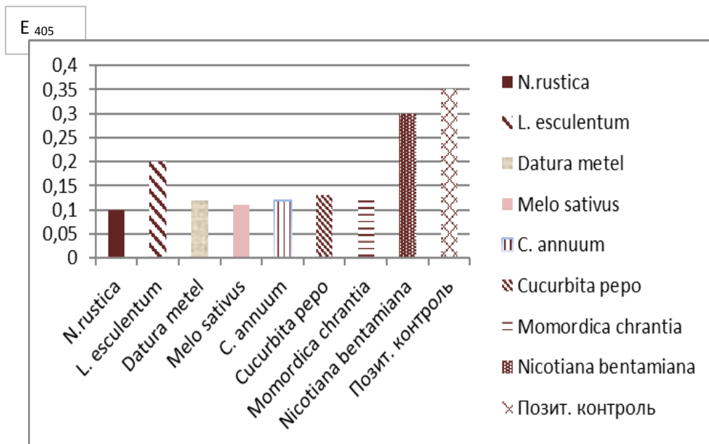
Fig. 2. ELISA results for HVX diagnostics in indicator-plants
