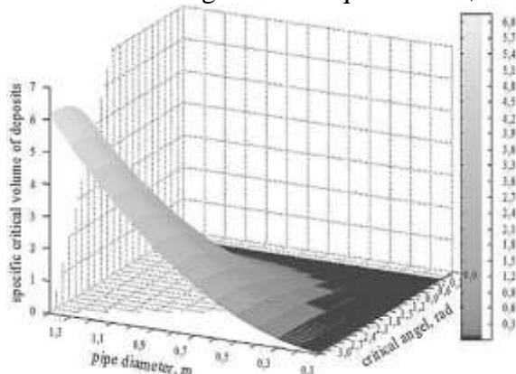
Fig. 6. Dependence of the liquid accumulation critical volume on critical angle φ and the pipeline diameter
