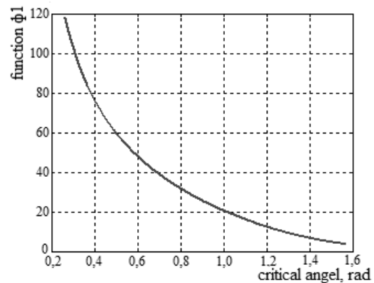
Fig. 4. Functional conditions \Phi_1(\phi_{cr}) curve
