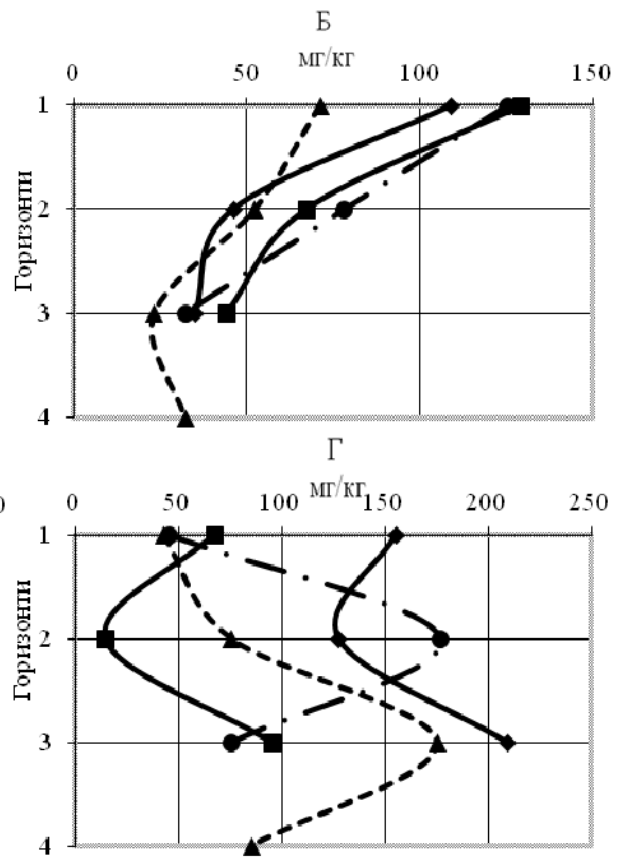
Fig. 2. Division of selected indicators by the soil type in Cheremosh National Park
