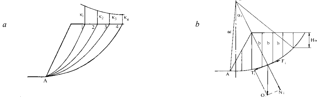
Fig. 3. Schemes of slope stability design by W. Terzaghi: a – hypothetical cylindrical sliding surfaces; b – method of segments; 1–4 are potential sliding surfaces and k_1 – k_4 – safety factor values; O – center of cylindrical arc; R – radius of the sliding surface; \alpha – angle between vectors of vertical and normal loads at certain segment b ; H_{90} – height of vertical slope failure
