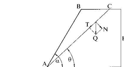
Fig. 1. Scheme of the slope failure with plane sliding surface by P.M. Tsimbarevich: ABC is the prism of the rock; AC – the line of plane sliding surface; H – height of the slope; N – normal forces; T – shearing forces; \alpha – angle of the slope inclination; \theta – angle of sliding surface inclination
