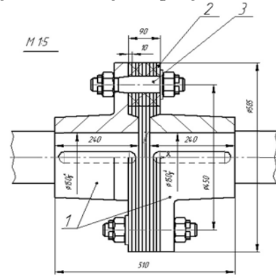
Fig. 4. The semi rigid coupling with steel disks
