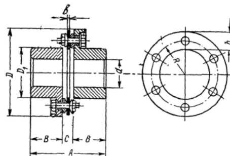
Fig. 4. The semi rigid coupling with steel disks
