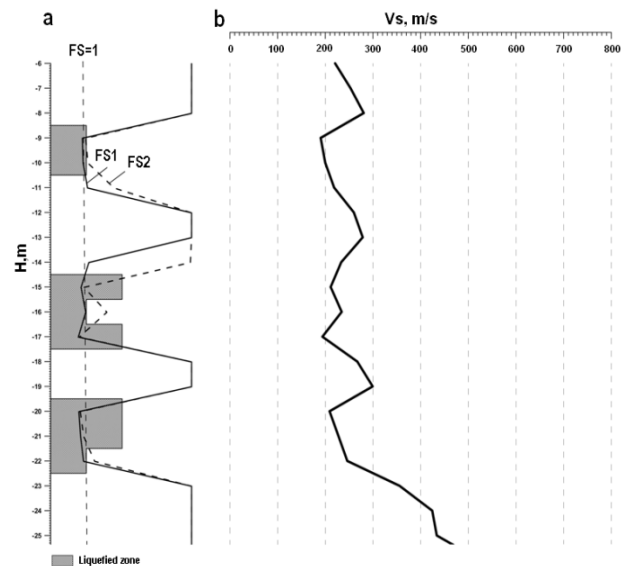
Fig. 7. Forecast of tectogenic soil liquefaction zones based on the vertical seismic profiling: a – the graph of changes in the factor of safety FS with depth; b – the graph of changes in the shear wave velocity Vs
