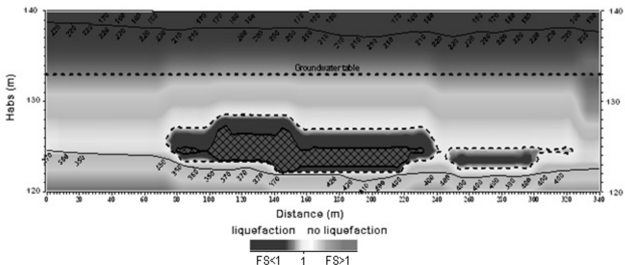
Fig. 8. Forecast of liquefaction of tectogenic soils by the materials of field seismology
