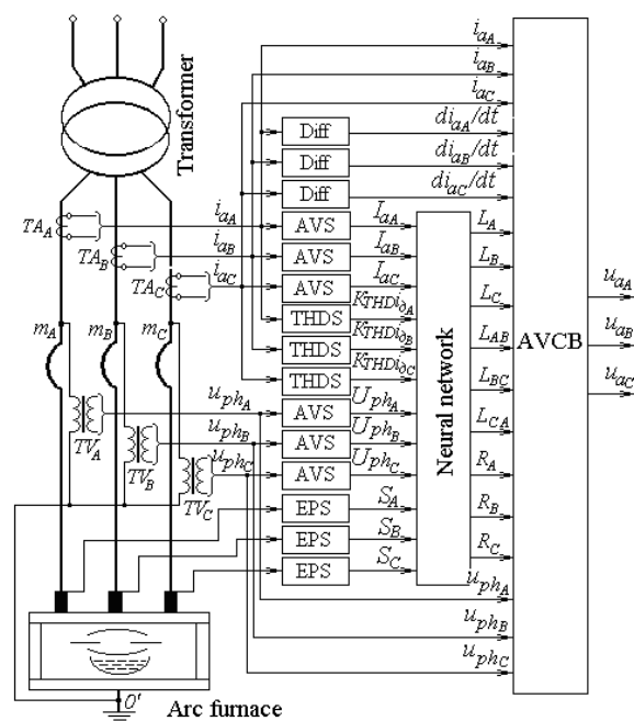
Fig. 1. Functional diagram of the block for real-time estimation of LVC parameters and EAF arc voltages
