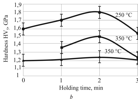
Fig. 3. Dependence of hardness of electric (a) and plasma coatings (b) on the holding time at pre-recrystallization heat treatment:
