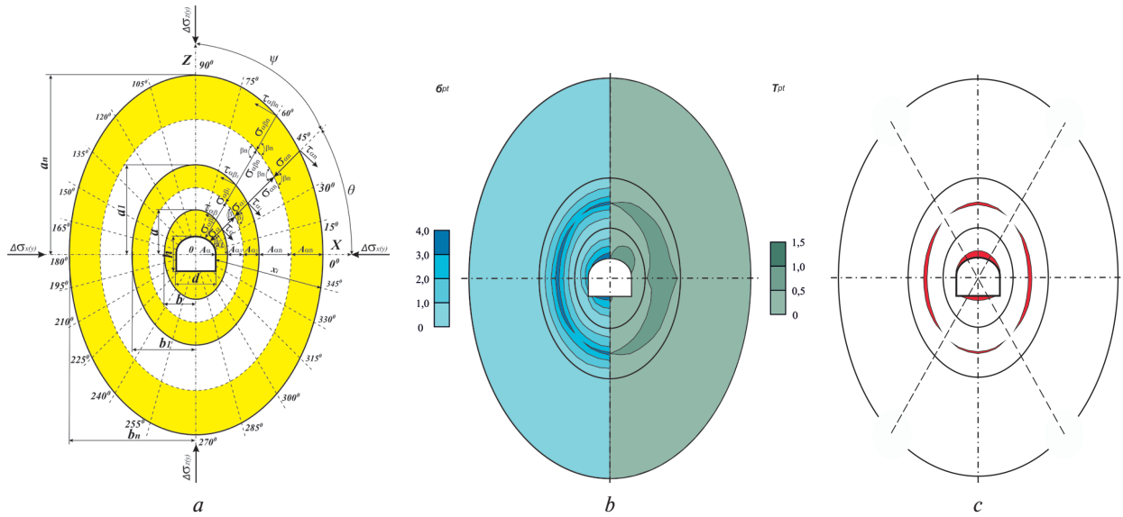
Fig. 2. The scheme to calculation of parameters of safety capsule created around development mine working (a) fields of radial \sigma_{pt} and tangential \tau_{pt} of total stresses in the massif of zones of thermodynamic energy balance, MPa (b) [14], formation of areas of massif deformation in zones of a thermodynamic energy disbalance (c, highlighted background) [14]
