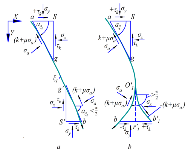
Fig. 2. Equilibrium triangles at TMETS \xi_1 , given that:
