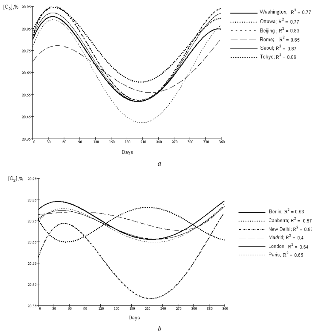
Fig. 1. Graphs of behavior of the calculated value of the oxygen volume concentration during 2014 in the main cities of the world:
