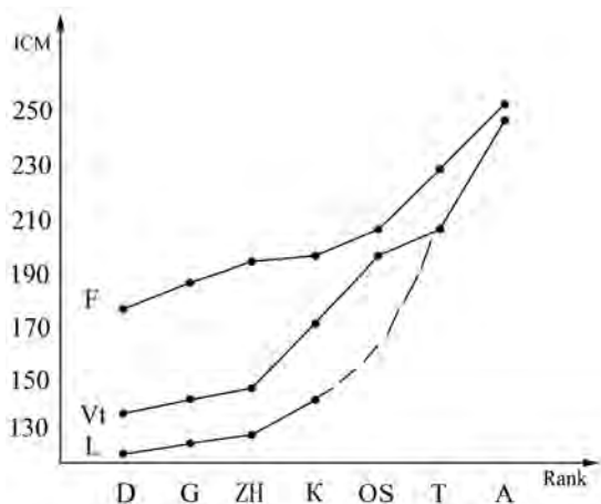
Fig. 6. The change in the intensity index of the gray color in a series of metamorphism for various macerals: F – fusinite; Vt – vitrinite; L – liptinit
