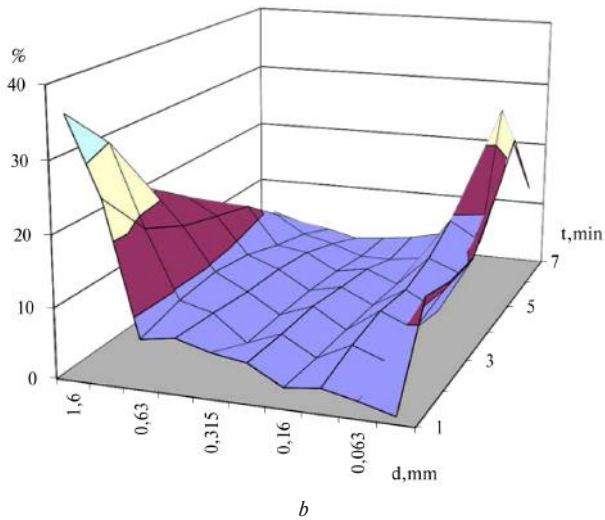
Fig. 2. Kinetics of fraction (1.0 + 0.63) of fireclay in the experimental grinding
