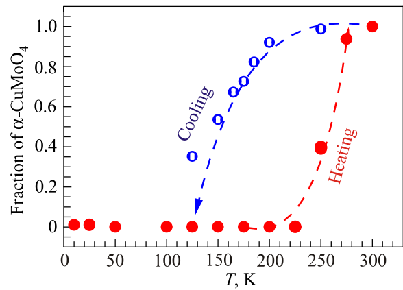
Fig. 3. Temperature dependence of the fraction of \alpha - \text{CuMoO}_4 phase upon heating (solid circles) and cooling (open circles).
