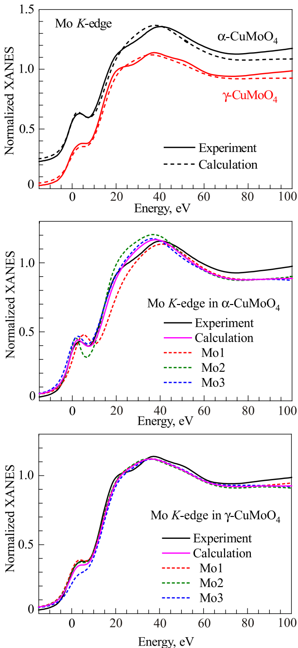
Fig. 4. (Color online) Comparison of the experimental and calculated Mo K -edge XANES of \alpha - \text{CuMoO}_4 and \gamma - \text{CuMoO}_4 phases (upper panel). Contributions from three non-equivalent molybdenum atoms (Mo1, Mo2, Mo3) to the Mo K -edge XANES are also shown in the middle and lower panels for \alpha - \text{CuMoO}_4 and \gamma - \text{CuMoO}_4 phases, respectively.
