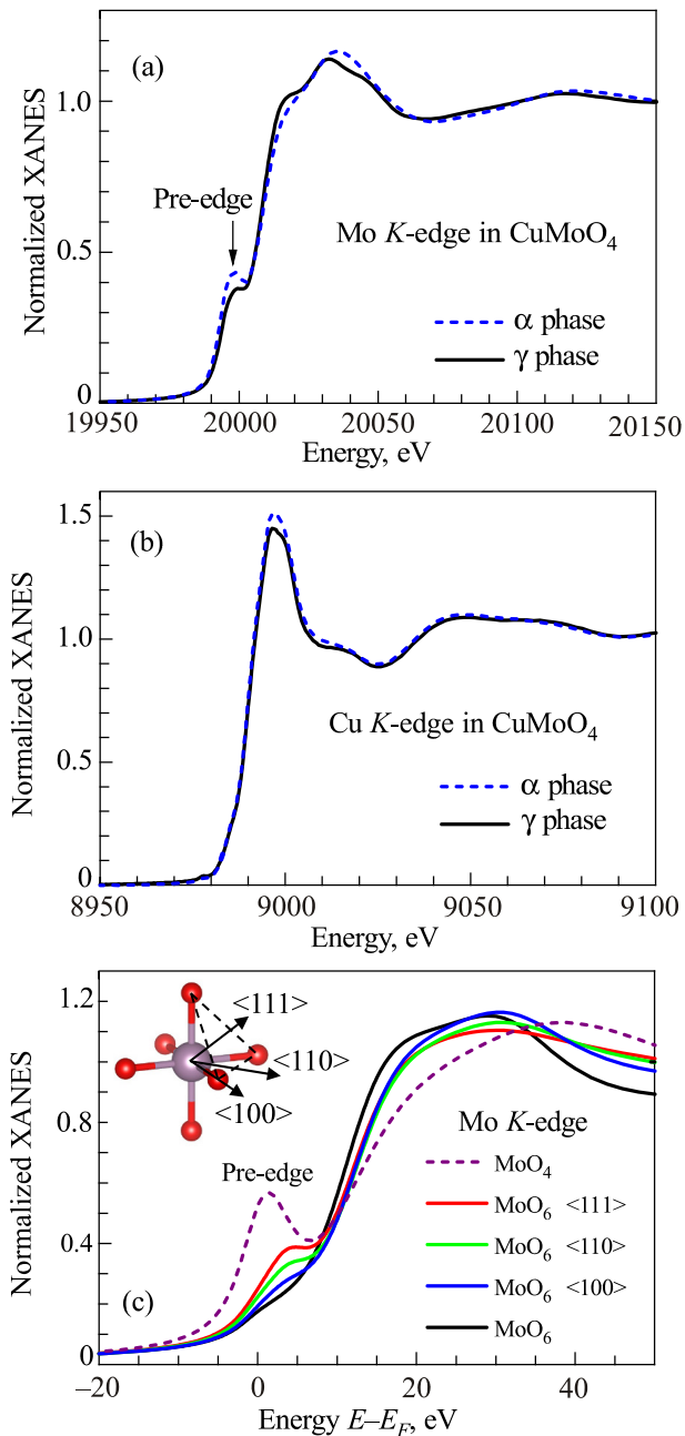
Fig. 2. (Color online) (a),(b) Experimental Mo and Cu K -edge XANES of \alpha - \text{CuMoO}_4 (at 300 K) and \gamma - \text{CuMoO}_4 (at 10 K) phases. (c) Calculated Mo K -edge XANES for regular \text{MoO}_4 tetrahedron, distorted and regular \text{MoO}_6 octahedra. Numbers in brackets indicate the direction of molybdenum ion off-center displacement. See text for more details.
