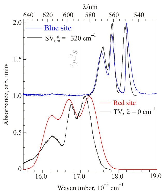
Fig. 4. (Color online) A comparison of the experimental absorption spectra — colour coded for the red and blue sites — with the band shapes simulated (black traces) for the SV and TV sites of Na/Xe. The experimental blue site band was recorded after annealing, while the red site was obtained as a difference spectrum of the freshly deposited and annealed scans. The band shown for the red site is the fit done on the difference spectrum with three Gaussian curves and presented in Fig. 1. In making this comparison with experiment, the simulated bands were generated at an effective temperature of 50 K as outlined in the Methods section. The SV and TV bands have been blue shifted by 1350 and 280 \text{cm}^{-1} respectively to match the observed bands. As indicated, the value of the spin-orbit coupling used for the SV site was \zeta = -320 \text{cm}^{-1} , while it was zero for the TV site.
