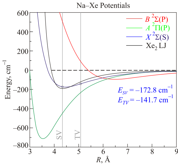
Fig. 2. (Color online) The potential energy curves for the ground X and excited A and B states of NaXe used in the spectral simulations of Na/Xe matrices. The origin of the curves are the ab initio calculations of Ref. 20 which are fitted to get the potentials shown. For the purposes of comparison the interaction potential of xenon dimer is also presented. A Lennard-Jones function, with the parameters \epsilon = 191.3 \text{ cm}^{-1} and \sigma = 3.88 \text{ \AA} , was used for \text{Xe}_2 . Shown by the vertical lines are the sizes of the single vacancy (SV) and tetravacancy (TV) sites in solid xenon. This comparison reveals how well the SV site size and the NaXe X state bond lengths match and the extent to which the TV site is too large.
