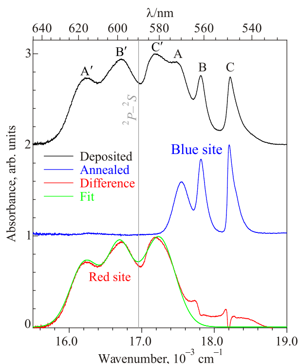
Fig. 1. (Color online) Absorption spectra recorded at T = 12.7 K for atomic Na isolated in a solid xenon matrix. The top panel shows the spectrum on deposition while that in the middle presents the blue site bands recorded after annealing the matrix to 35 K. In the bottom panel the red site spectrum, obtained as the difference of the freshly deposited and annealed scans, is shown by the red curve. As is evident by the complex structure in the blue portion of the difference spectrum, lineshape changes of the blue site occur on annealing. To obtain the isolated red site profile the results of a fit, done with three Gaussian curves is shown by the green trace. The vertical line indicates the position of the atomic Na 3p\ ^2P \leftarrow 3s\ ^2S transition in the gas phase.
