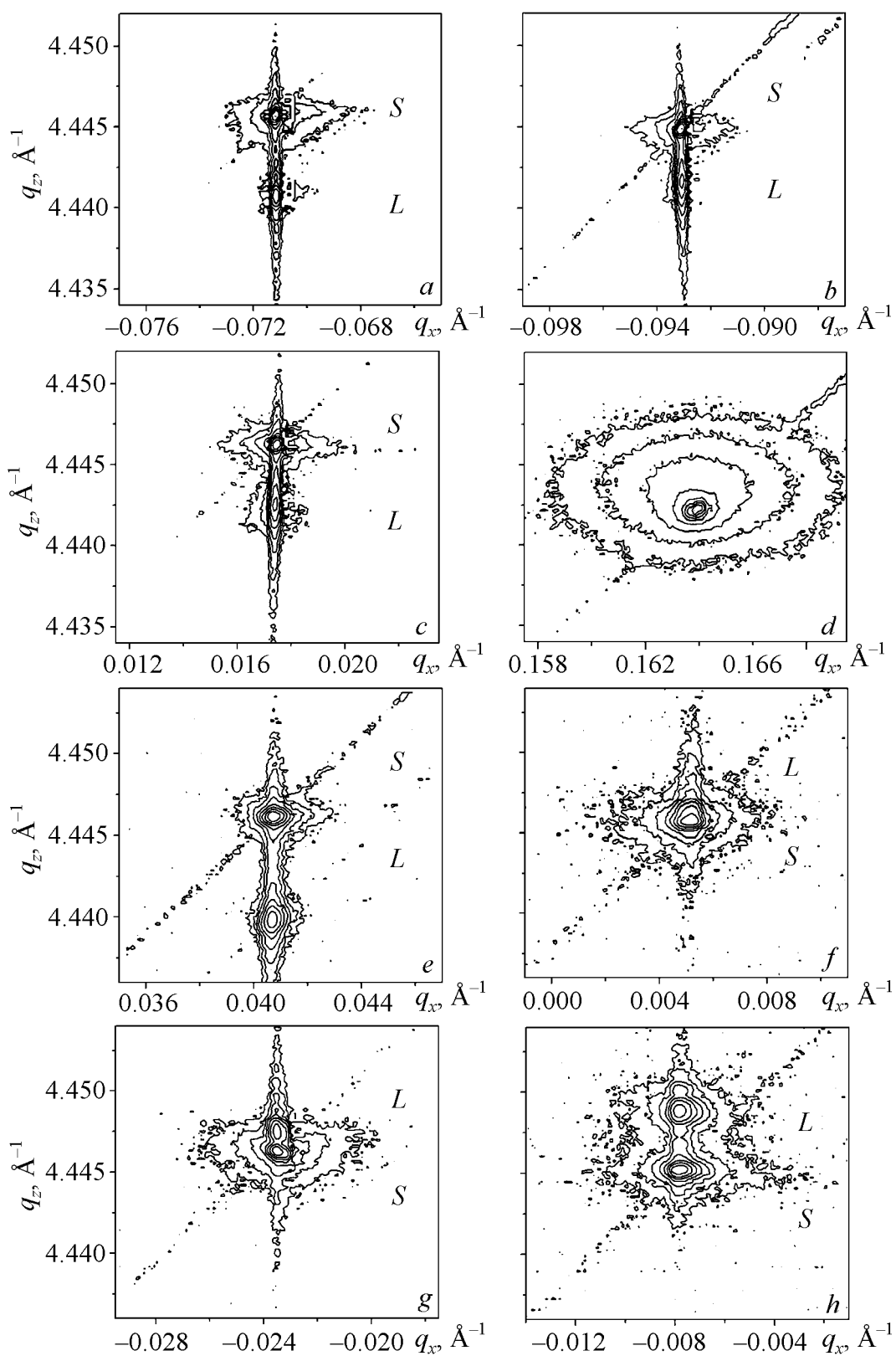
Fig. 5. 004 Reciprocal space maps of sample Ia ( a, b, c, d ) and of sample II ( e, f, g, h ): a, e – as-grown; b, f – annealed at HT = 650 \text{ K} - 10^5 \text{ Pa} ; c, g – treated at HT = 650 \text{ K} - 1.1 \text{ GPa} ; d, h – treated at 670 \text{ K} - 10^5 \text{ Pa} + 920 \text{ K} - 1.1 \text{ GPa}
