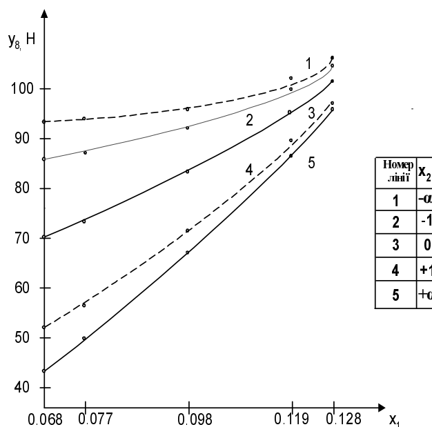
Fig. 1. Influence of Ludipress substance to resistance to crushing of Vispulin tablets
