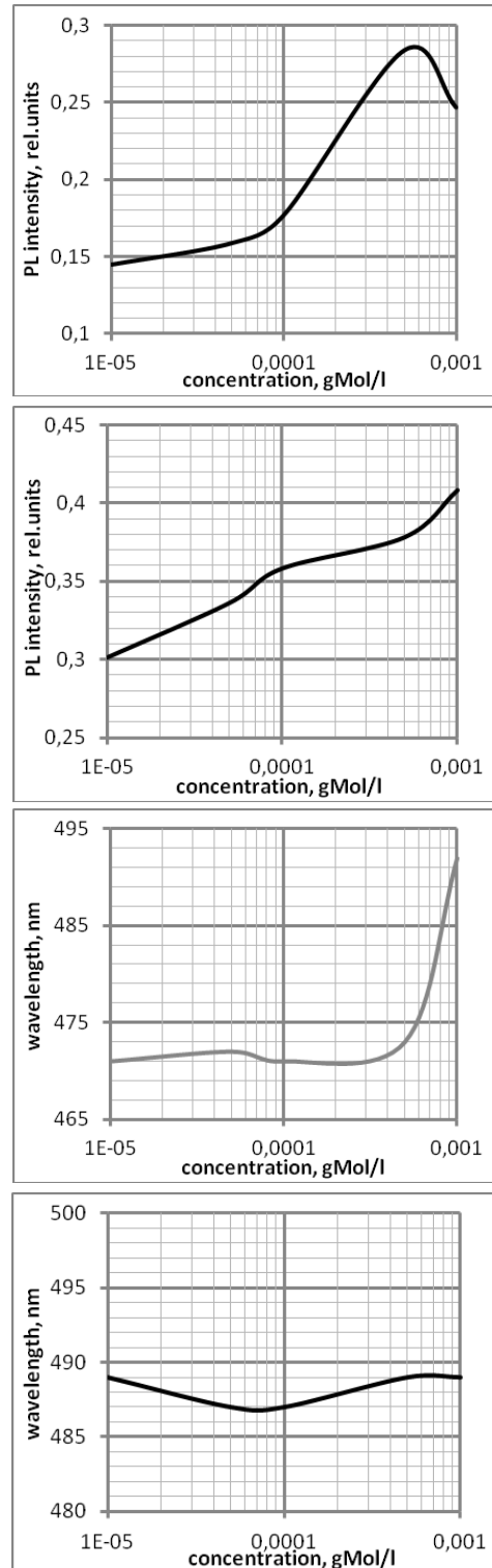
Fig. 3. Experimental concentration dependence of parameters of photoluminescence of nanoparticle ensemble of dye (I) (on the left) and dye (II) (on the right) in silica porous glass matrix
