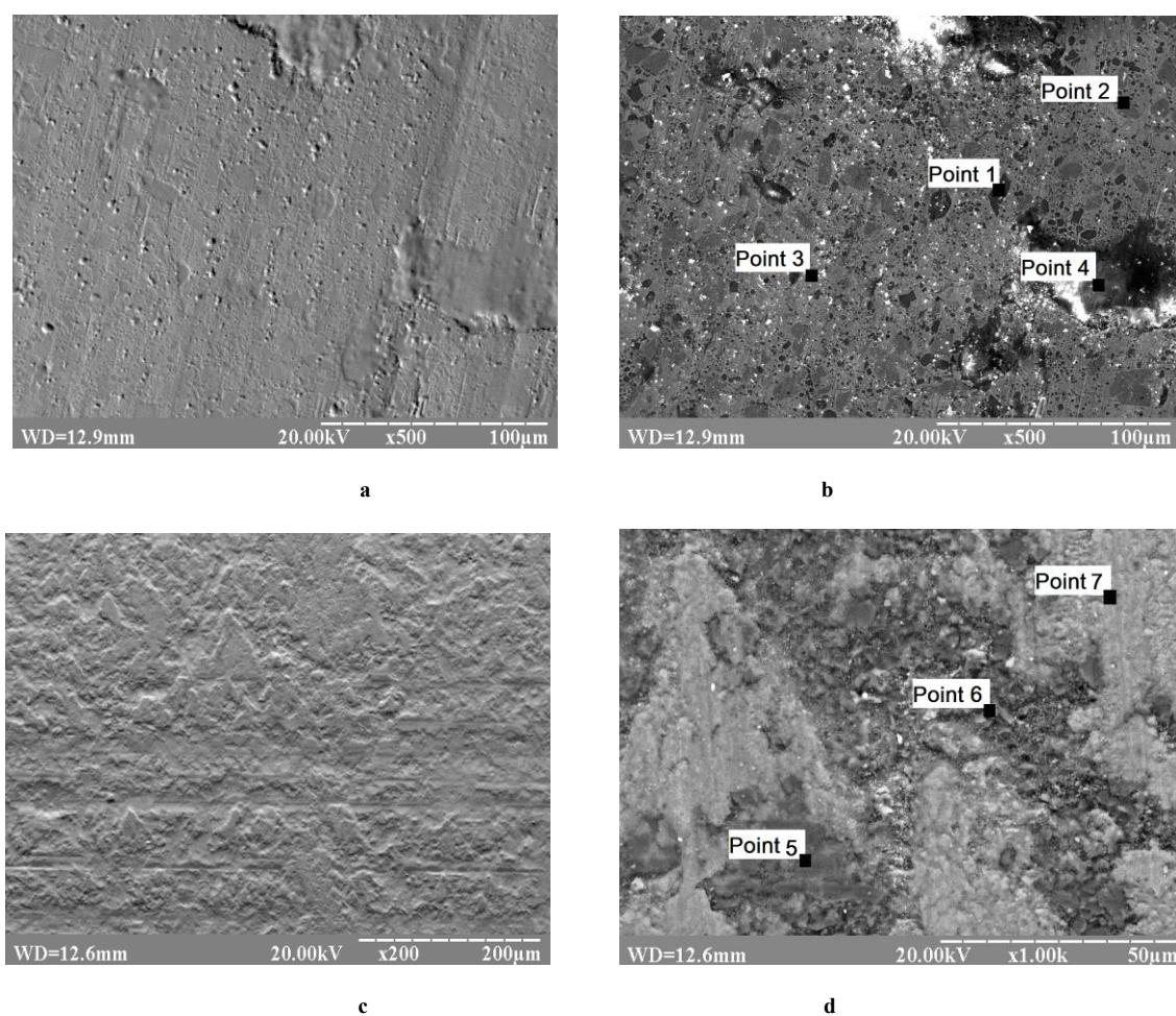
Fig. 5 – Morphology and microstructure of worn surfaces of NTB20-Al 2 O 3 tribocouple: a, b – worn surface of NTB20-coated pin; c, d – worn surface of Al 2 O 3 -coated disc
