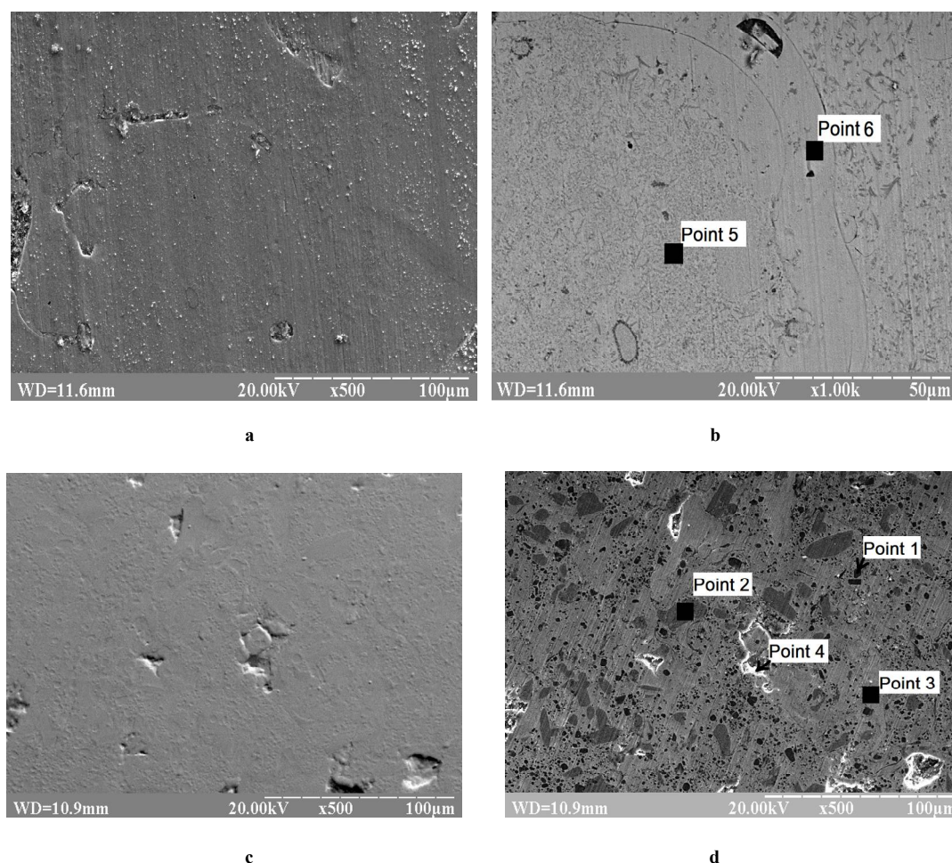
Fig. 4 – Morphology and microstructure of worn surfaces of NTB20-NiCrSiB tribocouple: a, b – worn surface of NTB20-coated pin; c, d – worn surface of NiCrSiB-coated disc
